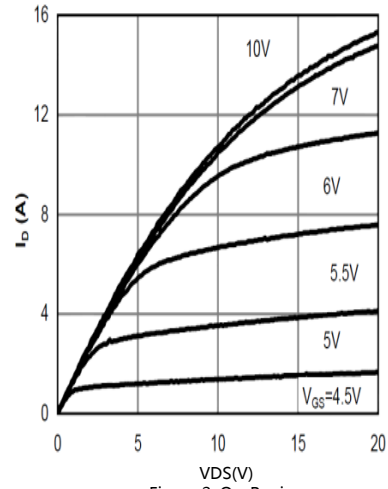
Figure 2: On-Region Characteristics@125°C
