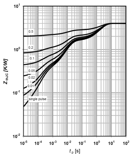
Figure 13: Maximum Transient Thermal Impedance
