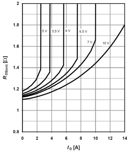
Figure 6: On-Resistance vs. Drain Current, T J =125°C
