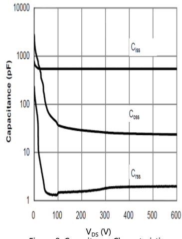
Figure 8: Capacitance Characteristics
