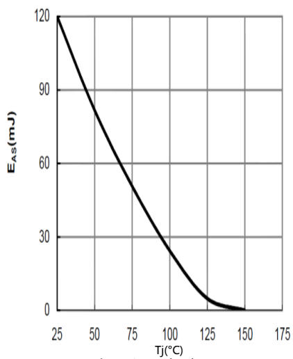
Figure 14: Avalanche energy
