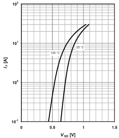
Figure 6: Body-Diode Characteristics
