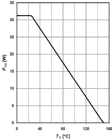
Figure 4 : Power dissipation
