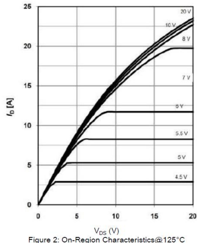
Figure 2: On-Region Characteristics@125°C
