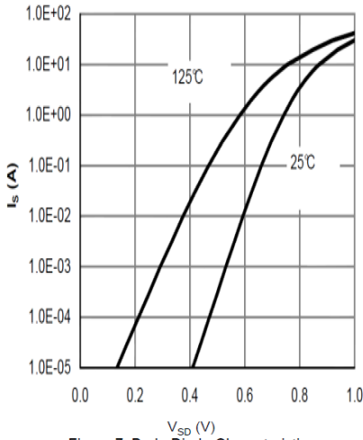
Figure 7: Body-Diode Characteristics
