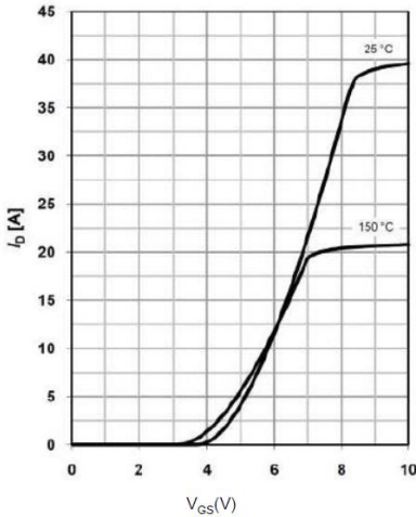
Figure 3: Transfer Characteristics
